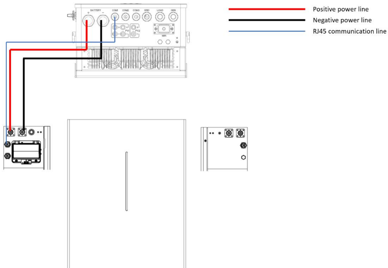
Two batteries connected to inverter
