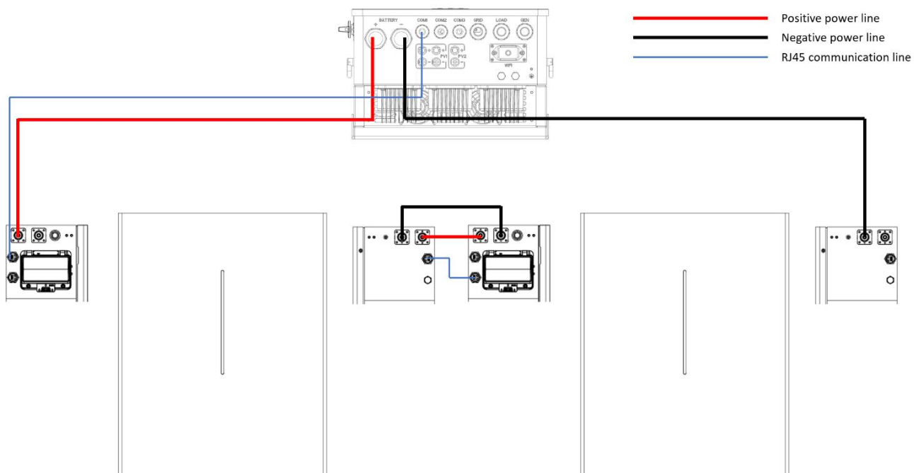
Three batteries connected to inverter
